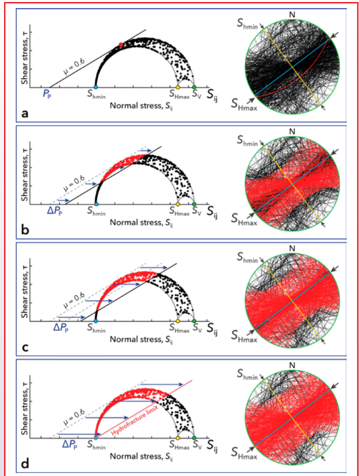
Figure 2: Mohr circles and stereonet plots illustrating the natural fractures measured in the FMI log that would be active at progressively increasing pore pressures during stimulation. a.–c. The number of fractures that will potentially fail in shear (red planes) increases as the pore pressure perturbation ( \Delta P_p ) increases. d. The fractures that are expected to slip once P_p reaches the frac gradient (“Hydrofrac limit”).
