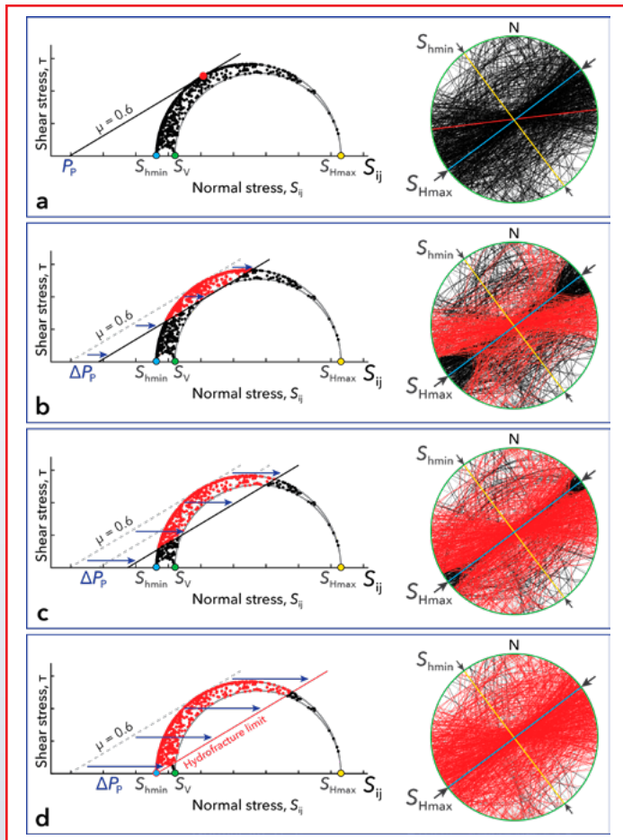
Figure 4: Mohr diagrams and stereonets showing which planes would be expected to slip if stimulation had instead occurred in a strike-slip/reverse faulting stress state.
