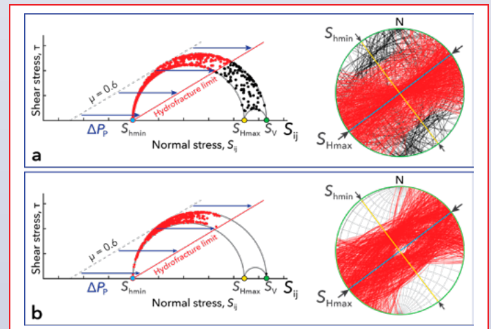
Figure 3: a. Plots showing the fractures identified in the FMI log. Planes colored red would be expected to slip during stimulation at pore pressures sufficient to propagate a hydraulic fracture. b. Plots of the orientations of planes that actually slipped during stimulation. These orientations were generated by sampling from a distribution of active faults from microseismic focal mechanisms with noise applied to represent orientation uncertainties.
